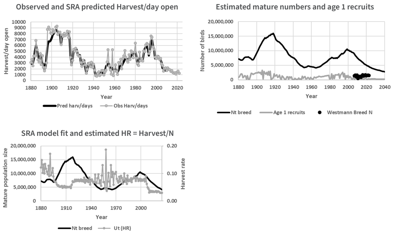
Figure 2. Model fit diagnostics for the total Iceland age-structured population model; note that harvest data after 2010 made it possible to fit the model to a longer time series of relative abundances. Black dots in the top right panel show direct estimates of Westmann breeding numbers from number of nesting holes and occupancy rates.
