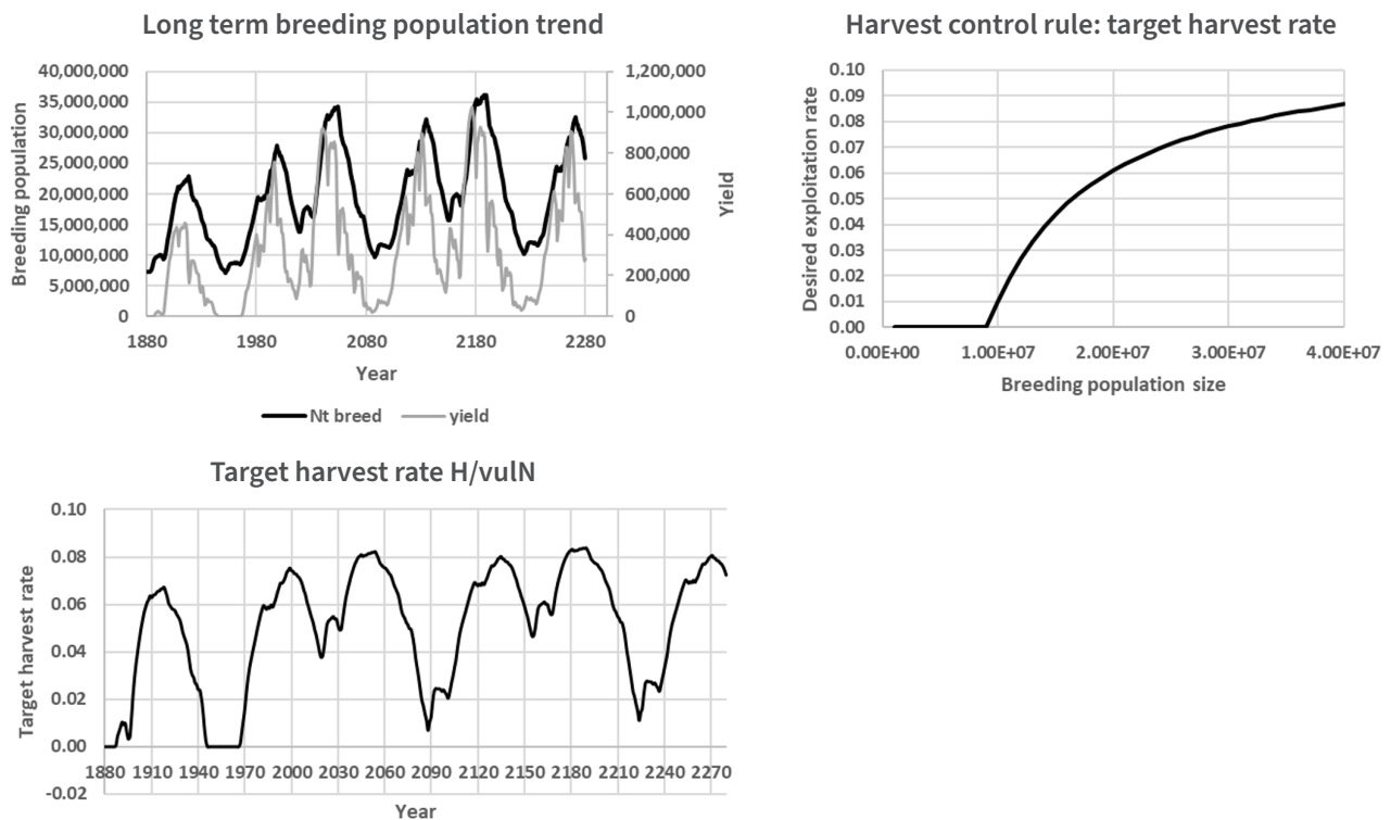
Figure 4. Results from very long term (400 year) simulations with the total Iceland population fitted model, where estimated historical productivity anomaly patterns are repeated every 130 years and where exploitation rates are managed starting in simulation year 1880 using a harvest control rule that maximizes predicted total long-term utility of the harvest. Note that the harvest control rule would have stopped all harvesting over the 1950-70 period of low productivity, possibly not a socially or legally viable option.
