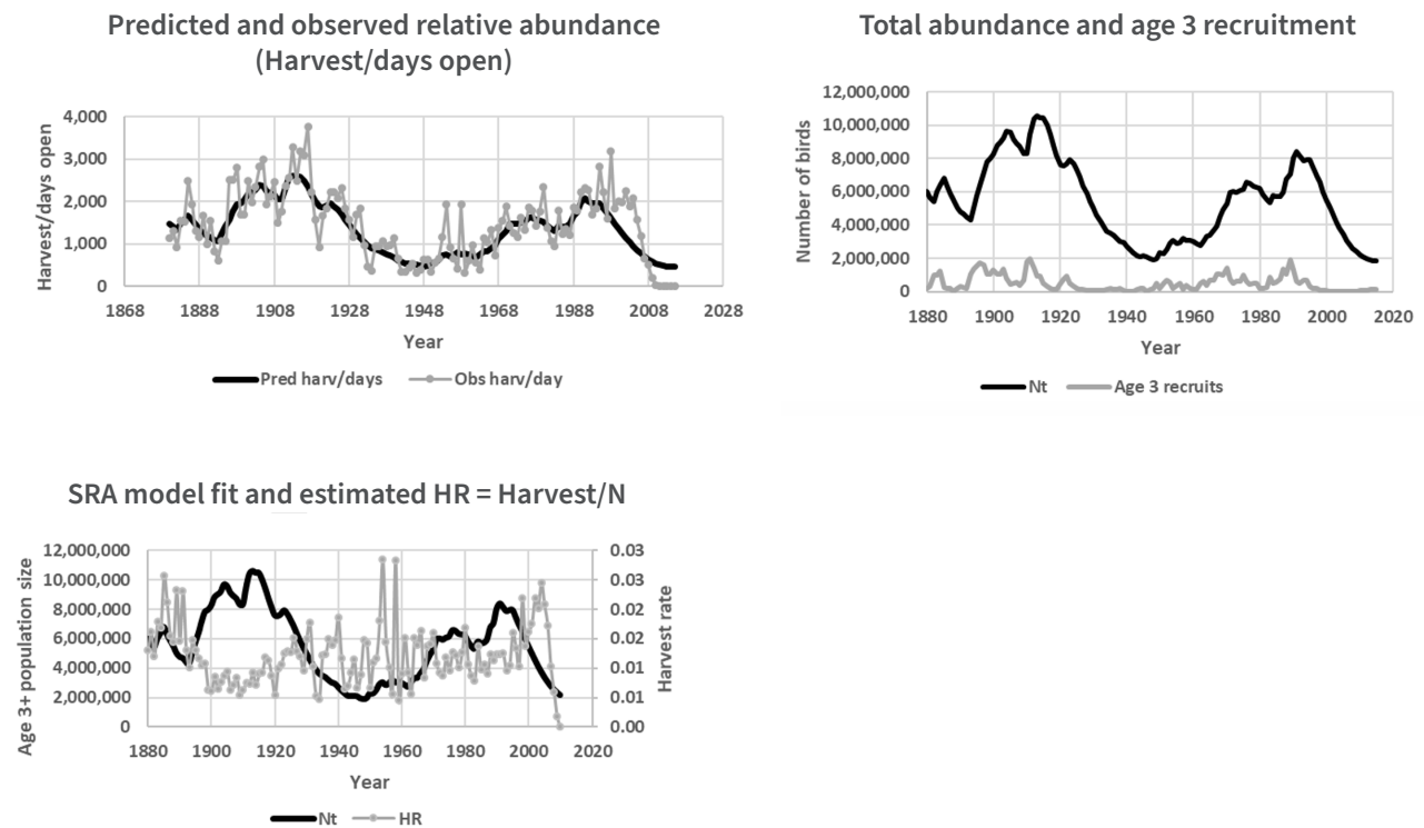
Figure 3. Model fit diagnostics for the simple balance model. For these fits, reproductive rate parameter B was frozen at 0.135 for the age model and was estimated to be lower for the balance model for recruitment to age 3 (0.11) as expected since births are multiplied by three rather than two years of survival rates.
